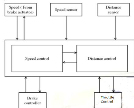
Fig.4 ACC signals and information flow
