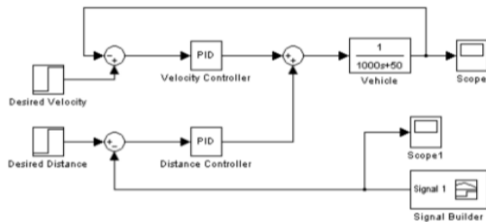
Fig5. A Trial ACC Simulation Model
