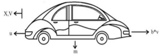
Fig.1. Free-body diagram of a car
